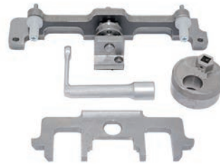
TATHT8286 Mercedes-Benz 651 Timing Chain Guide Tool
